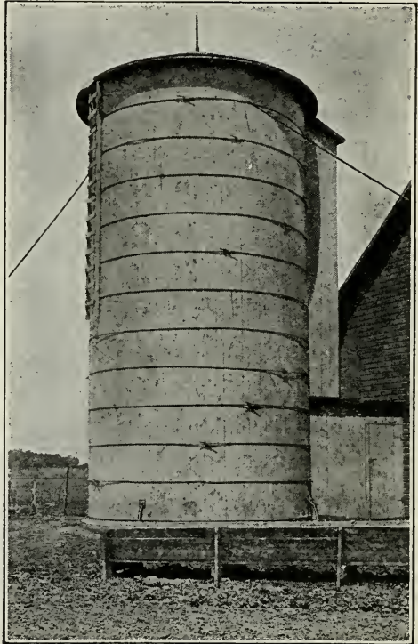
Fig. 294. A good stave silo well anchored.
