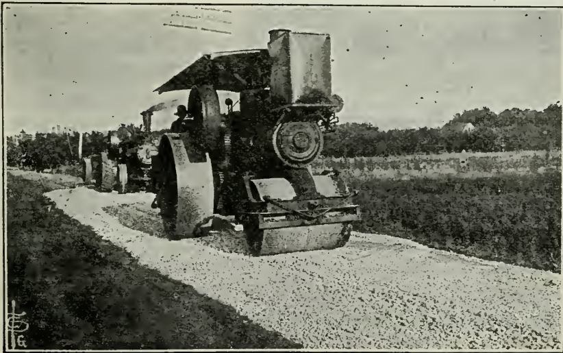
Fig. 84. Rolling the first course of stone.
