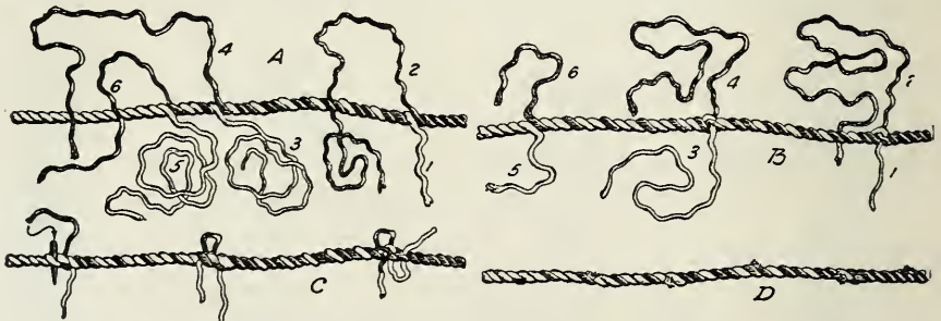
Fig. 340. Long splice, three-strand rope.
