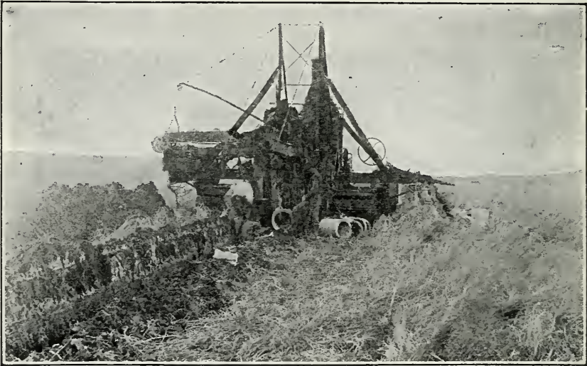
Fig. 55. A large tile ditching machine at work.
