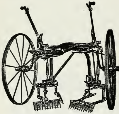
Fig. 150. A surface cultivator.
