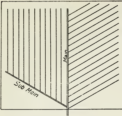
Gridiron System
