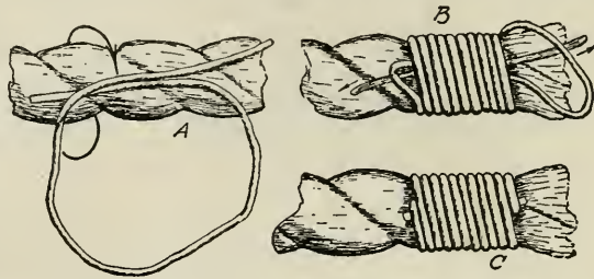
Fig. 337. Whipping.
