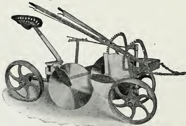
Fig. 116. A deep-tilling machine.
