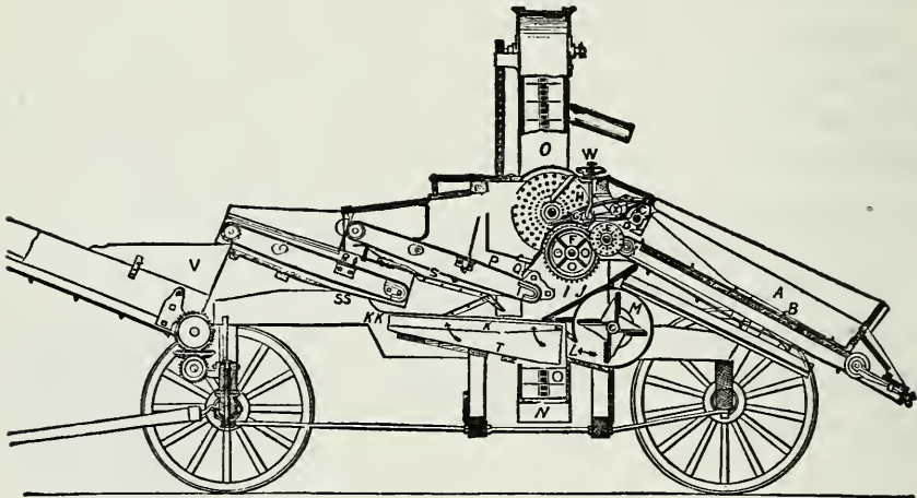
Fig. 190. A section of a picker-wheel sheller.
