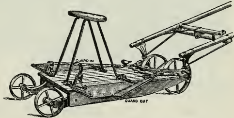
Fig. 156. A sled corn harvester.
