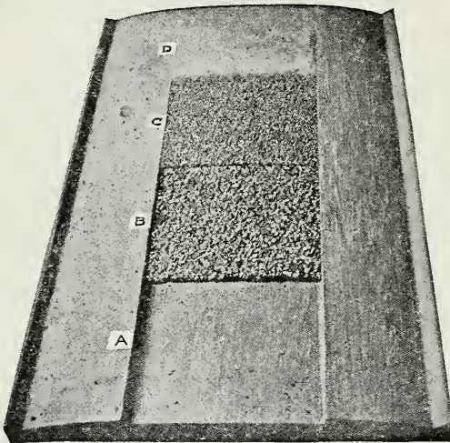
Fig. 85. Model of a water-bound macadam road. A represents the prepared subgrade. B represents the first course of coarse stone. C represents the second course of stone, chips or dust. D the finishing layer of stone, chips or dust. (Bul. 36, Office of Public Roads, U. S. Dept. of Agr.)
