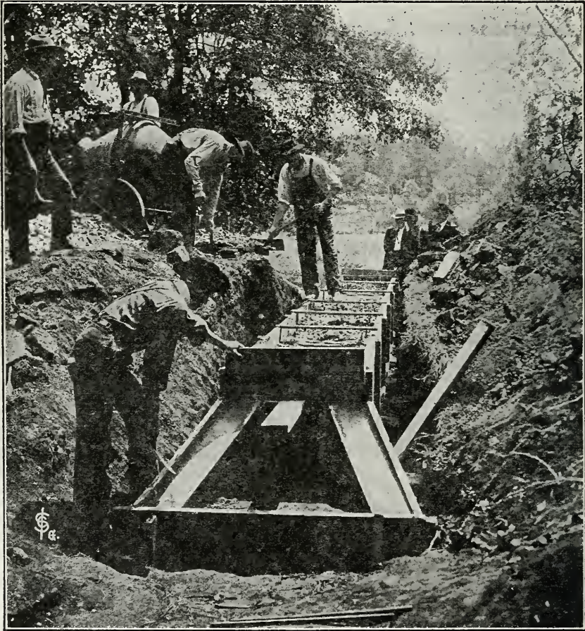
Fig. 95. Making a concrete culvert.
