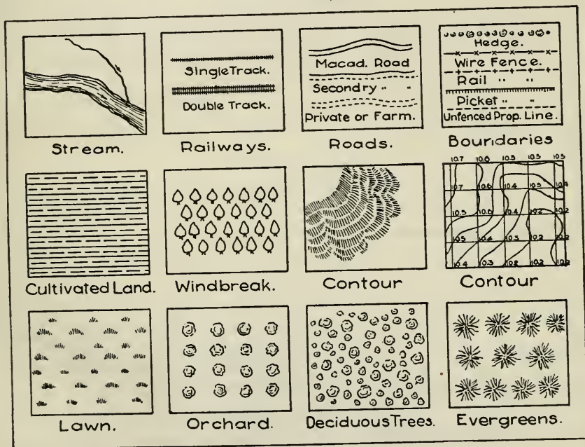
Fig. 13. Conventional topographical signs.
