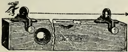
Fig. 33. A carpenter's level with sights attached.
