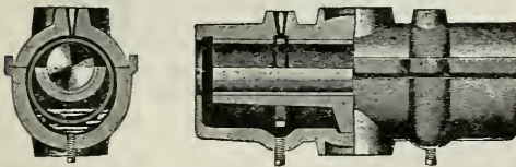
Fig. 104. A ring oiling bearing.
