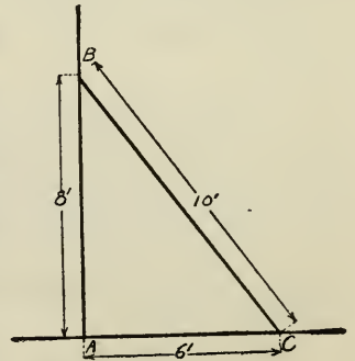
Fig. 7. Sketch showing how a line may be laid off at right angles to another at a point A.
