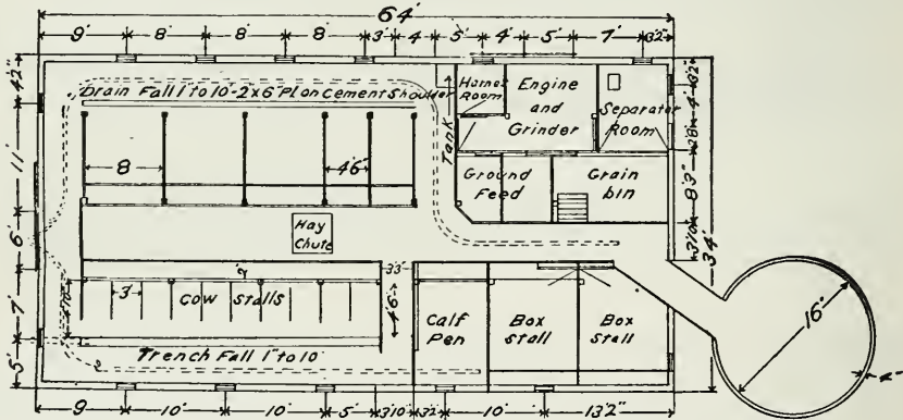
Fig. 284. Floor plan of a general farm barn.
