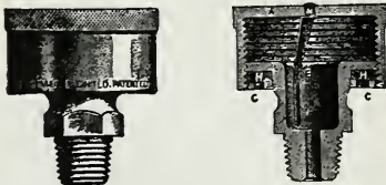
Fig. 107. A grease cup for feeding hard oil.
