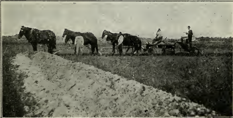
Fig. 62. Filling the ditch with a road grader.
