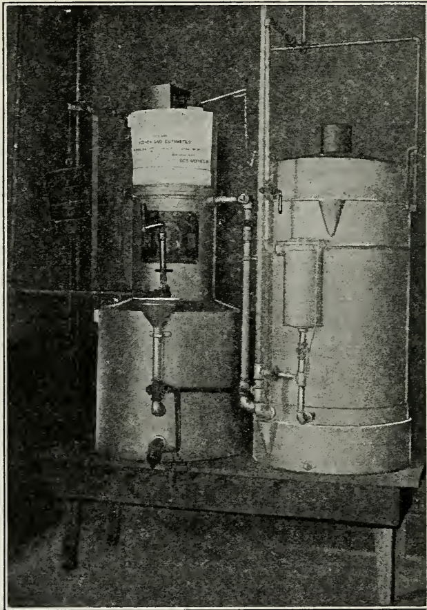
Fig. 315. A 35-light acetylene generator.
