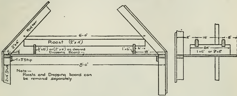
Fig. 274. Detail of roosts and dropping board.
