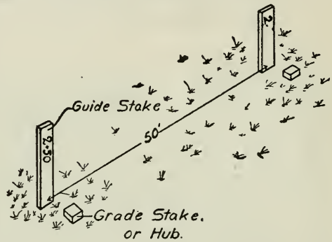
Fig. 49. Grade stakes, or hubs, and guide stakes.
