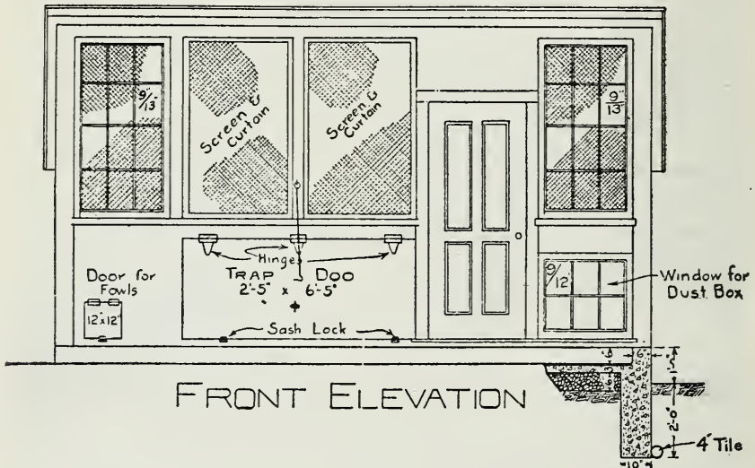
Fig. 278. Front elevation accompanying Fig. 277.
