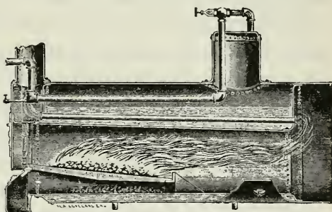
Fig. 242. A sectional view of a return-flue boiler.
