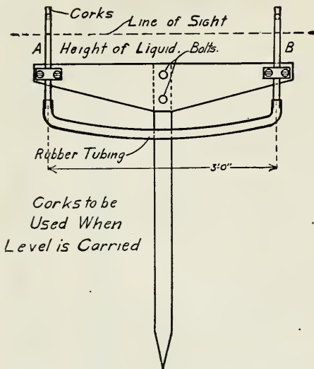
Fig. 31. A home made water level.
