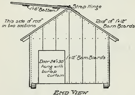
Fig. 265. End elevation of gable-roof colony hog house.
