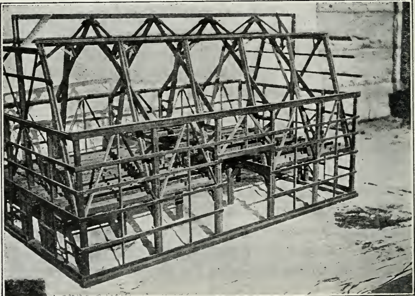
Fig. 288. A model Shawver barn frame.
