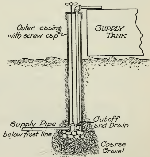
Fig. 306. A satisfactory method of installing exposed hydrants.
