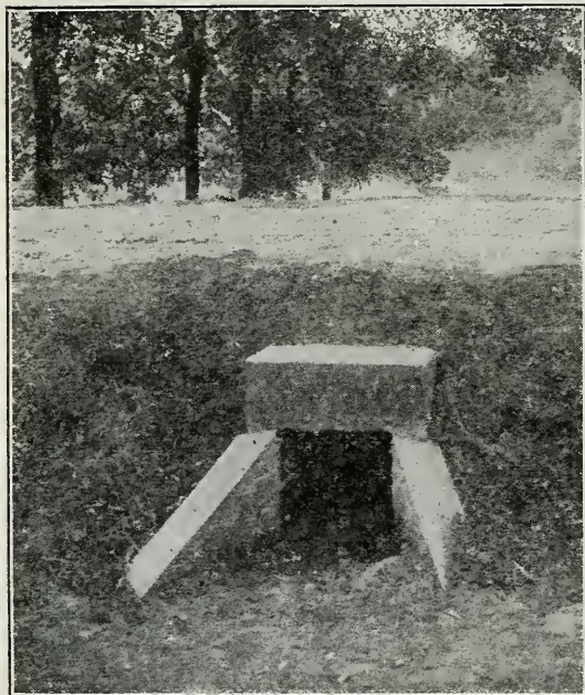
Fig. 97. Concrete culvert after the plan of Fig. 96.
