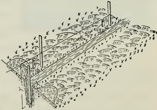
Fig. 56. The line method of grading tile ditches.
