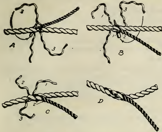
Fig. 341. Side splice.
