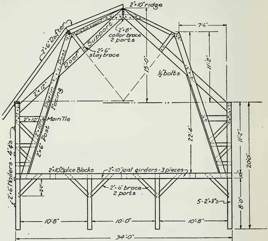
Fig. 290. A sketch of the Shawver barn frame.
