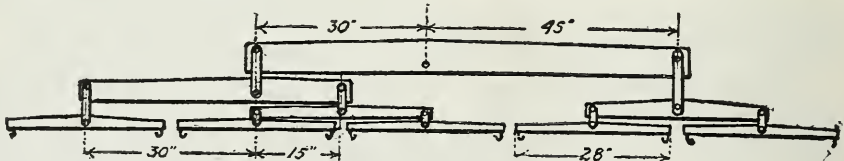
Fig. 216. A plain five-horse evener.
