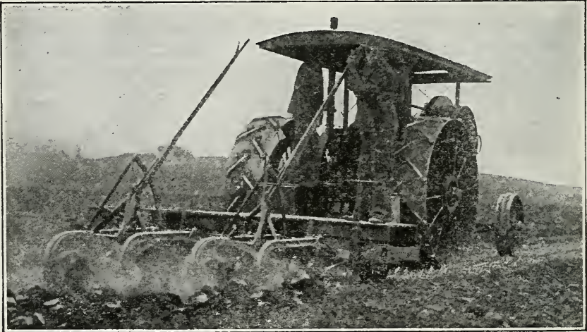
Fig. 236. A small gas tractor plowing. It may be successfully operated by one man.
