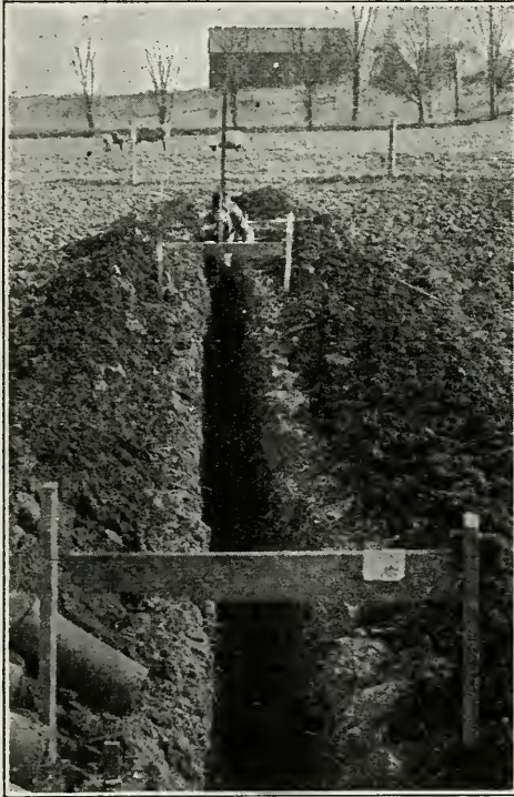
Fig. 57. The target method of grading tile ditches.
