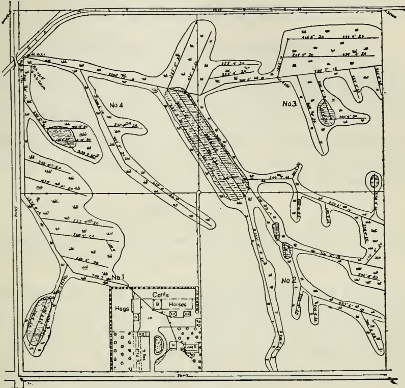
Fig. 52. A drainage map.
