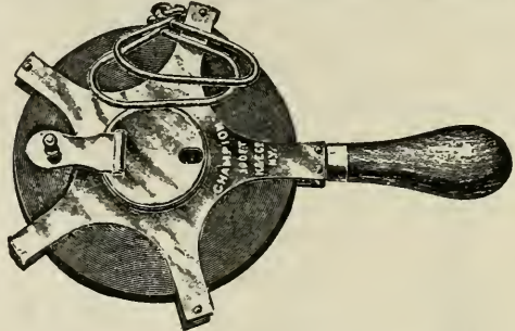
Fig. 3. A steel tape wound on a reel.
