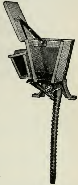
Fig. 141. A section of the seed box of a drill showing location of the grass seed box and a steel ribbon tube.
