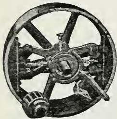
Fig. 238. One form of clutch. The wooden shoes are forced outward against the rim of the wheel, engaging it by friction.
