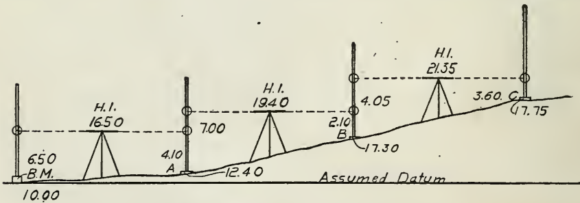
Fig. 38. Sketch illustrating the levels of Fig. 37.
