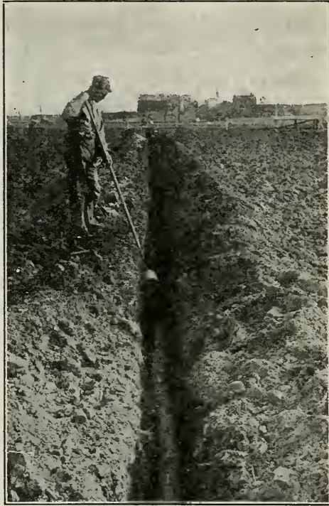
Fig. 59. Laying tile with the tile hook.
