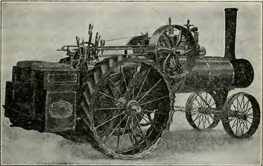
Fig. 252. A top-mounted steam tractor.
