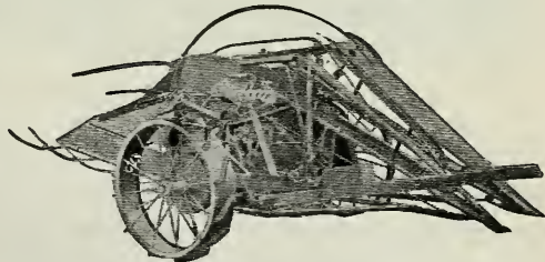
Fig. 158. A corn harvester of the horizontal type.
