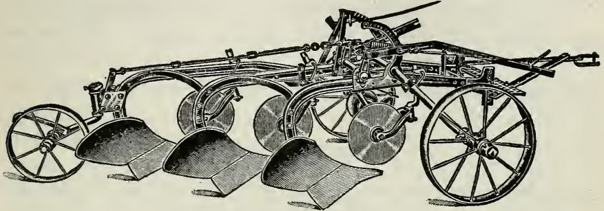
Fig. 118a. Rigid beam gang plow.
