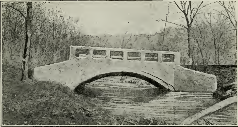
Fig. 98. A concrete bridge which failed on account of the foundation.
