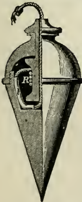
Fig. 30. A plumb-bob with line attached
