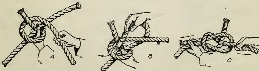
Fig. 327. Sheet bend, or weaver's knot.
