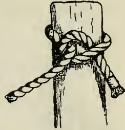
Fig. 331. Half hitch.
