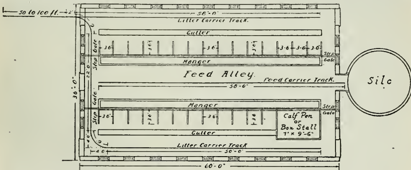
Fig. 281. Floor plan of a modern dairy barn.
