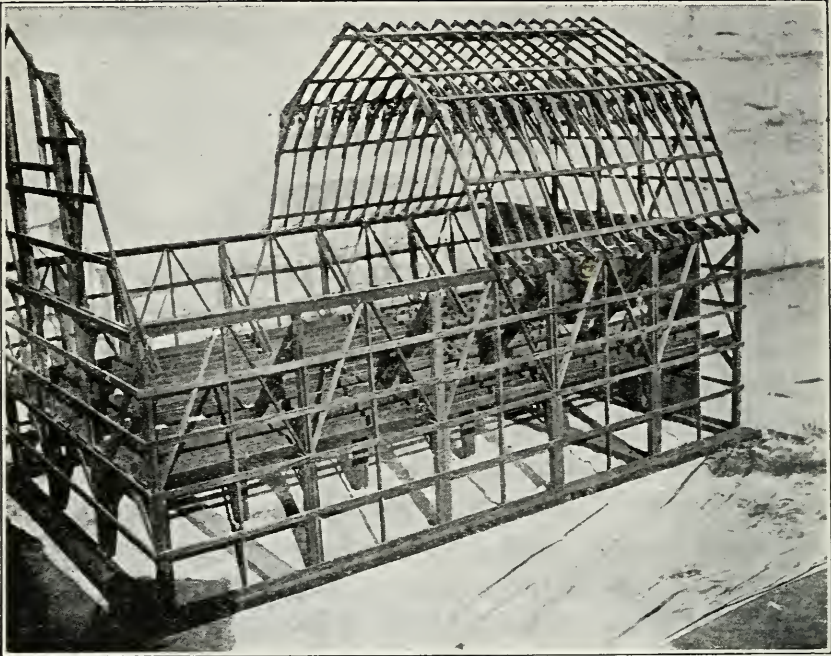
Fig. 287. A model Wing joist barn frame.
