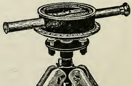
Fig. 34. An inexpensive farm level with horizontal circle for turning off angles.
