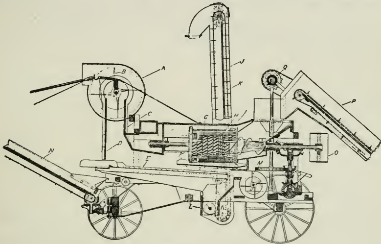
Fig. 191. A section of a cylinder sheller.
