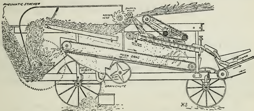
Fig. 161. A section of a corn husker and shredder.
