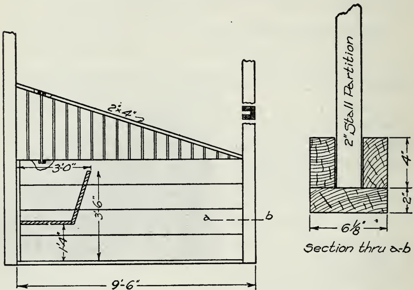
Fig. 286. Detail of construction of a horse stall.
