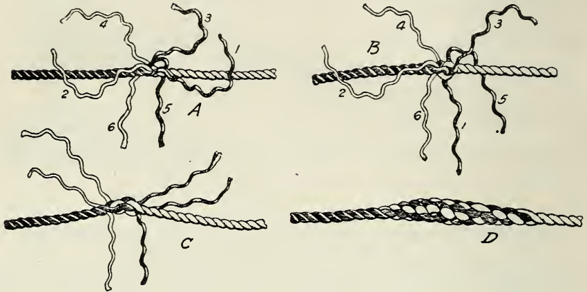
Fig. 339. Short splice.
