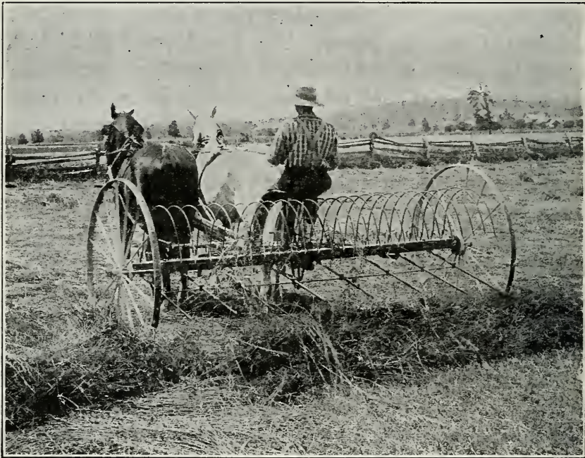
Fig. 165. A modern self-dump sulky rake at work.
