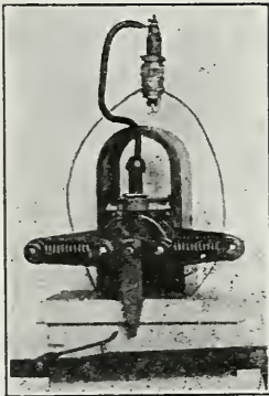
Fig. 231. An oscillating magneto on demonstration stand.
