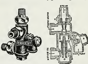
Fig. 245. A standard type of injector.
