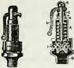
Fig. 243. A spring-loaded safety valve.
