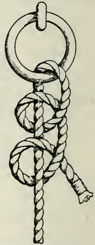
Fig. 335. Two half hitches.
