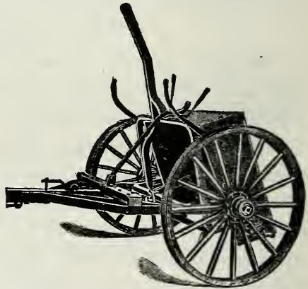
Fig. 90. Wheel scraper, dumped.
