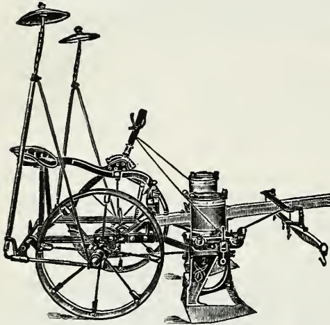
Fig. 144. A corn planter with stub shoe furrow-openers.
